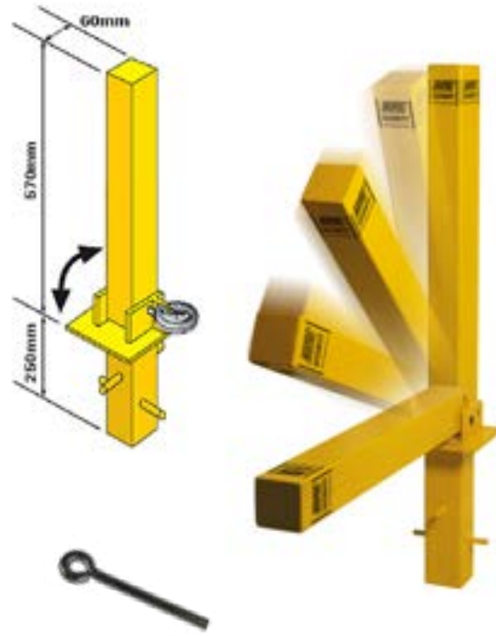
MP97371 - Spare eye pin
